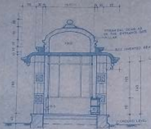
SECTION-XX
